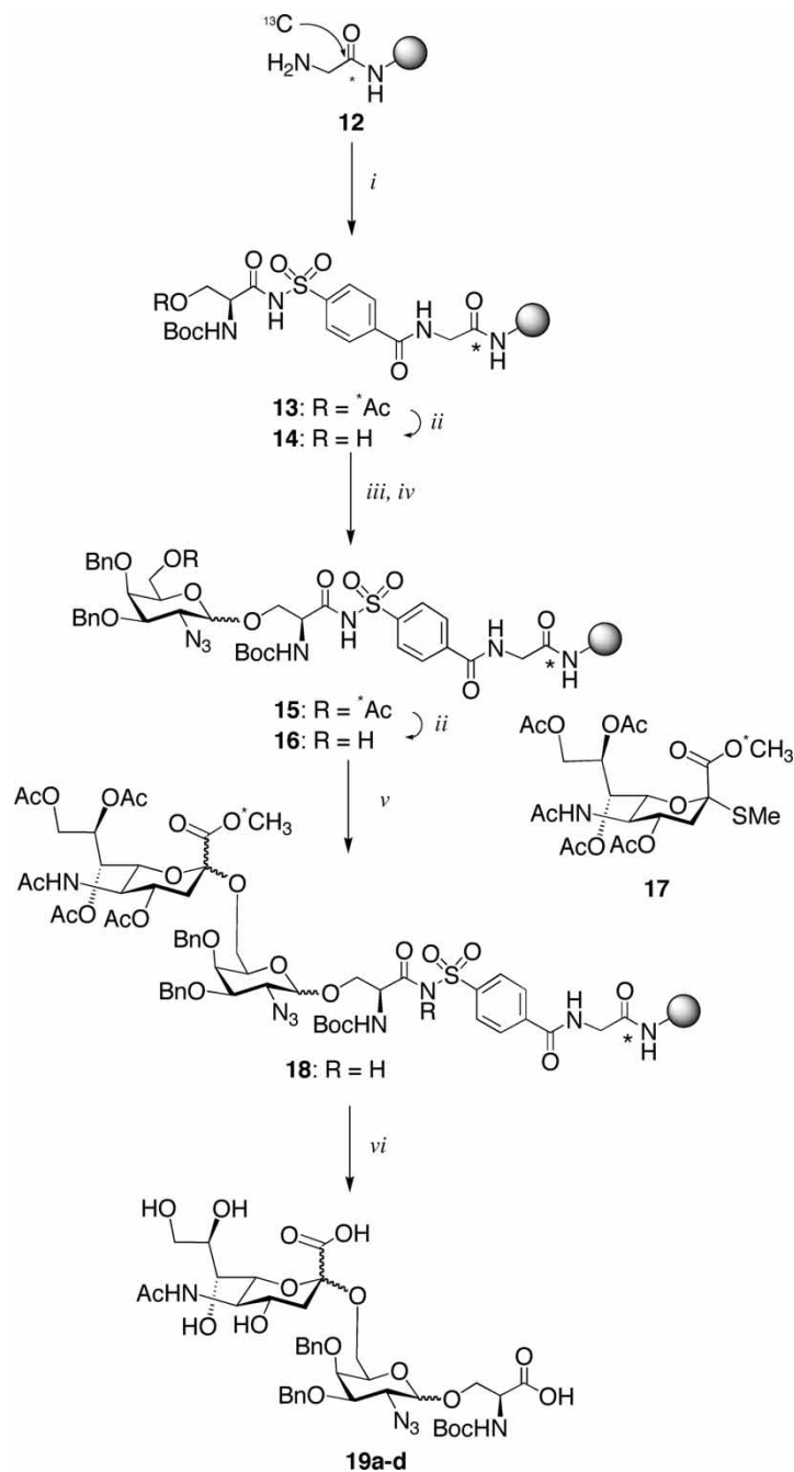
Scheme 3: Solid-phase synthesis of sialyl Tn antigen. i. 6 , DIPC-HOBT- i Pr 2 EtN/DMF, rt, 12 h, 97%; ii. 0.05 M NaOMe/MeOH-DMF (1:1), rt, 12 h, quant.; iii. 11 , DMTST/CH 2 Cl 2 -Et 2 O (1:1), 0°C, 12 h, twice, 82%; iv. TBDMSCl-imidazole / CH 2 Cl 2 , rt, 12 h; v. 17 , DMTST/CH 3 CN, -15°C, 12 h, twice, 80%; vi. a) TMS-diazomethane, i Pr 2 EtN/THF, rt, 24 h; b) 0.05 N NaOH/H 2 O-THF (1:1), rt, 12 h, 62% (in two steps).
