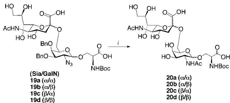
Scheme 4: Deprotection reactions. i. (a) \text{Pd}(\text{OH})_2\text{-H}_2/\text{MeOH-H}_2\text{O-AcOH} , rt, 12 h, (b) \text{Ac}_2\text{O} , pyridine, rt, 12 h, (c) 0.05M \text{NaOMe}/\text{MeOH} , r.t., 3 h.
