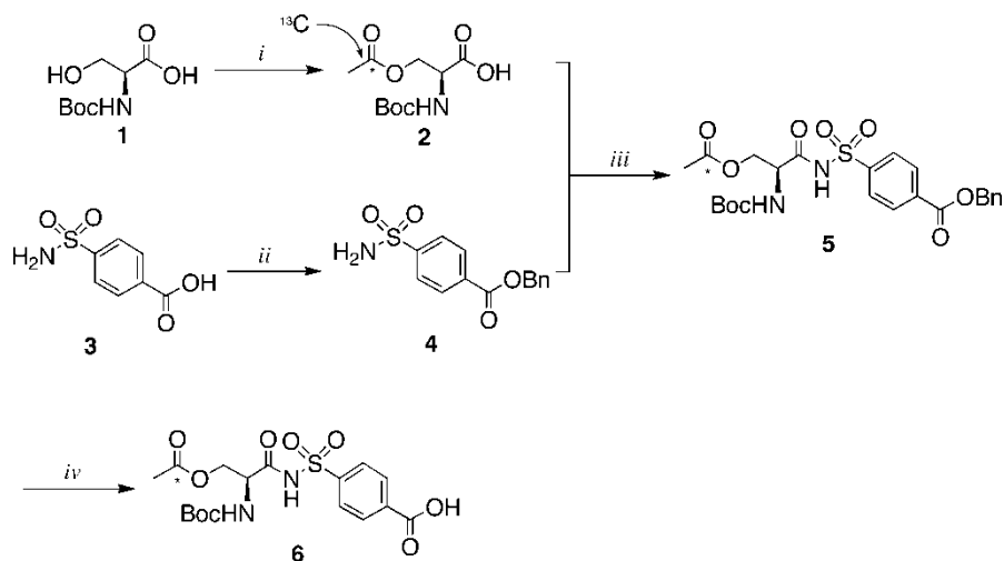
Scheme 1: Synthesis of L-Ser attached to the acylsulfonamide linker. i. acetic- 1\text{-}^{13}\text{C} anhydride, DMAP/ \text{CH}_2\text{Cl}_2 , rt, 12 h, 92%; ii. BnOH, DIPC, HOBT / DMF, rt, 12 h, 85%; iii. PyBop, \text{Pr}_2\text{EtN}/\text{CH}_2\text{Cl}_2 , -20^\circ\text{C} , 10 h, 72%; iv. 10% Pd/C, \text{H}_2/\text{MeOH} , rt, 12 h, 88%.
