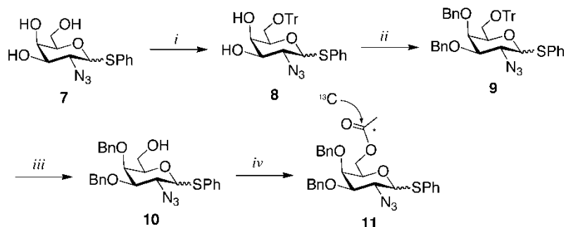
Scheme 2: Synthesis of GalN donor. i. TrCl, pyridine, rt, 24 h, 90%; ii. BnBr, NaH/DMF, rt, 2 h, 90%; iii. 10% TFA/CH 2 Cl 2 , rt, 1 h, 83%; iv. acetic- 13 C acid, DCC, DMAP/CH 2 Cl 2 , rt, 4 h, 94%.
