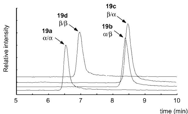
Figure 1: Chromatograms of purified compounds 19a–d .
